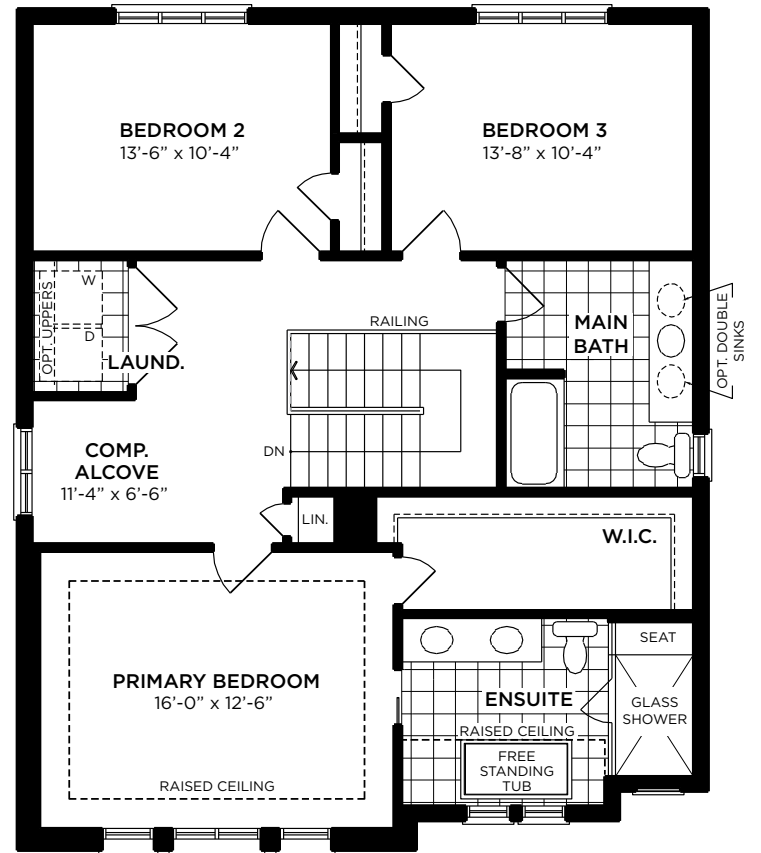
SECOND FLOOR PLAN Elev. A
