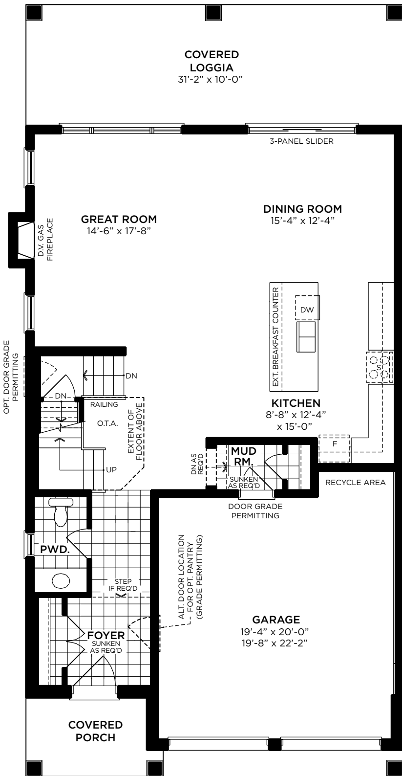
GROUND FLOOR PLAN Elev. A
