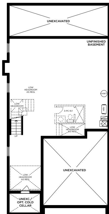
BASEMENT PLAN Elev. A
