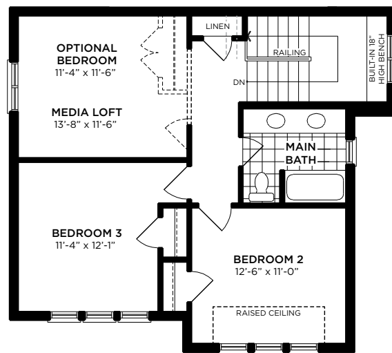
SECOND FLOOR PLAN W/ 3 BEDROOM & MEDIA LOFT Elev. A
